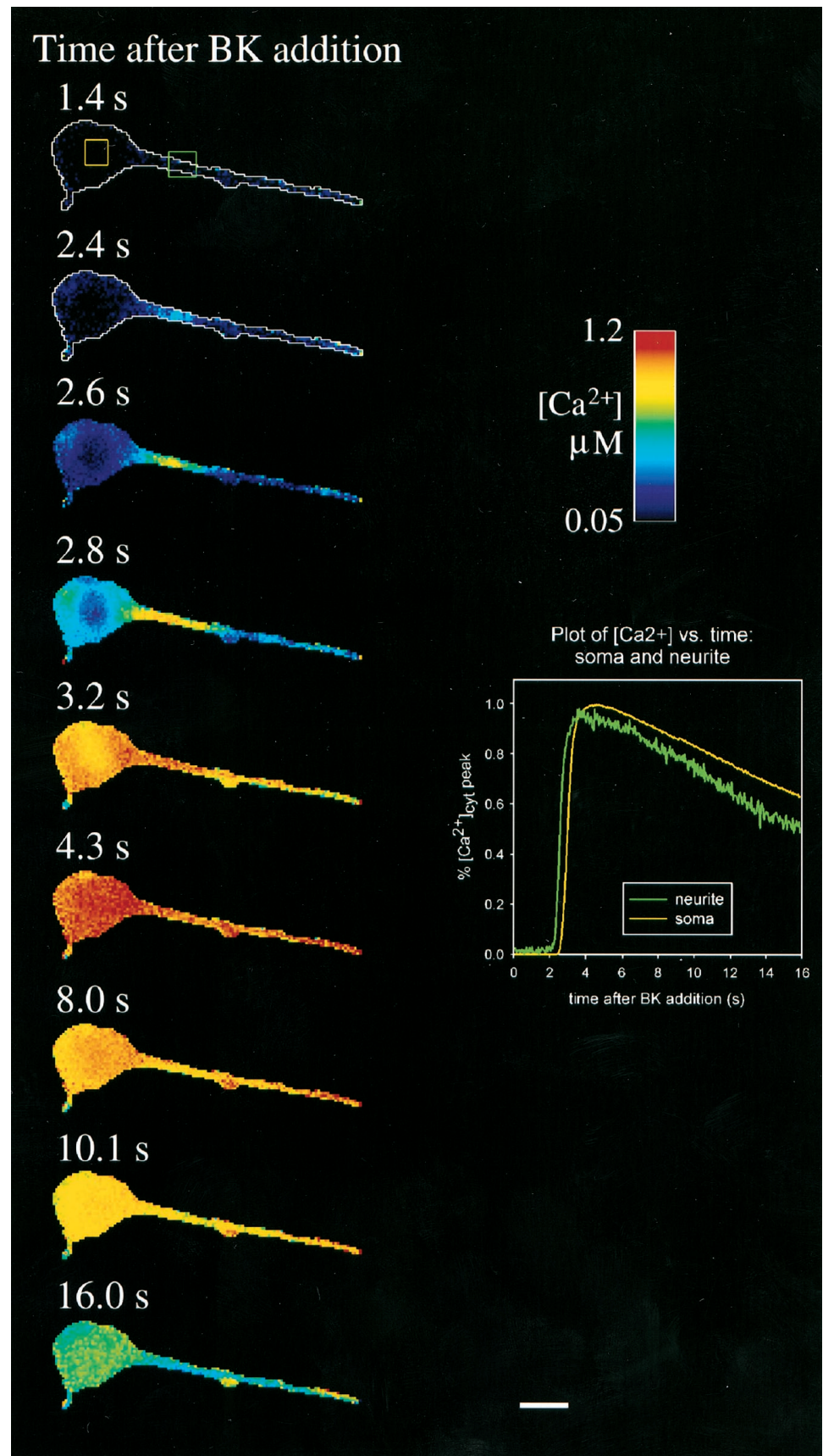
FIGURE 1 BK-induced calcium wave in an N1E-115 Nb cell. BK (500 nM) was externally applied to the bathing medium of a cell stained with fura-2. Fluorescence from the 380-nm excitation was collected with a cooled CCD camera, converted to [Ca 2+ ], and displayed in pseudocolored form. For regions of interest in the soma and neurite (indicated by the colored rectangles), the relative change in [Ca 2+ ] versus time was plotted in the lower right-hand corner. Scale bar = 25 μM.
