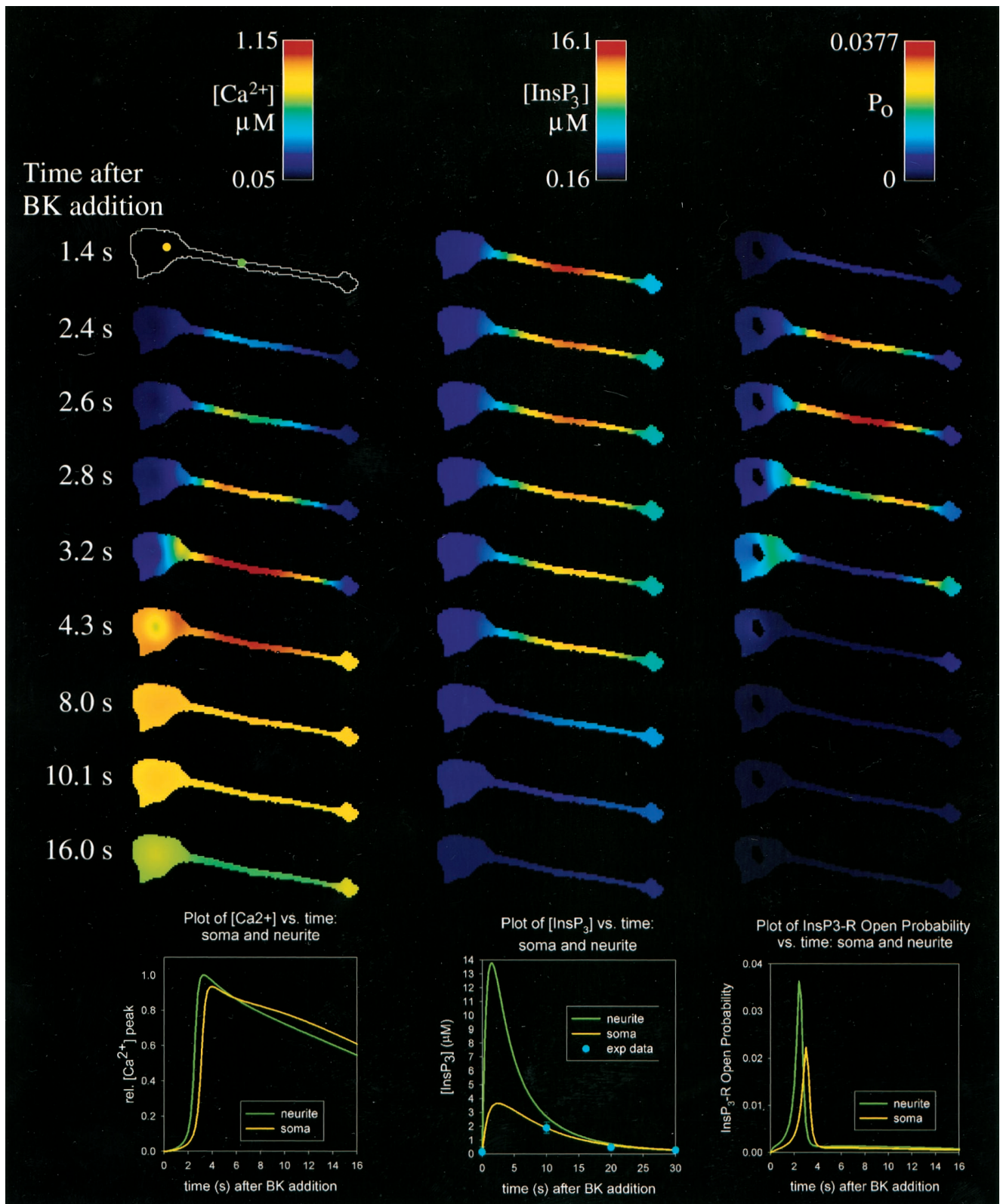
FIGURE 4 Simulation of BK-induced calcium wave using parameters illustrated in Fig. 3 b . From left to right columns, pseudocolored images show simulation results for [Ca^{2+}]_{\text{cyt}} , [InsP_3]_{\text{cyt}} , and P_O (the probability of opening of the InsP 3 -R). At the bottom of each column, values in the soma and neurite (indicated by the yellow and green dots in the 1.4 s [Ca^{2+}]_{\text{cyt}} image) are plotted against time. For the [InsP_3]_{\text{cyt}} versus time plot, experimentally determined data (filled cyan circles) are superimposed onto the simulation data.
