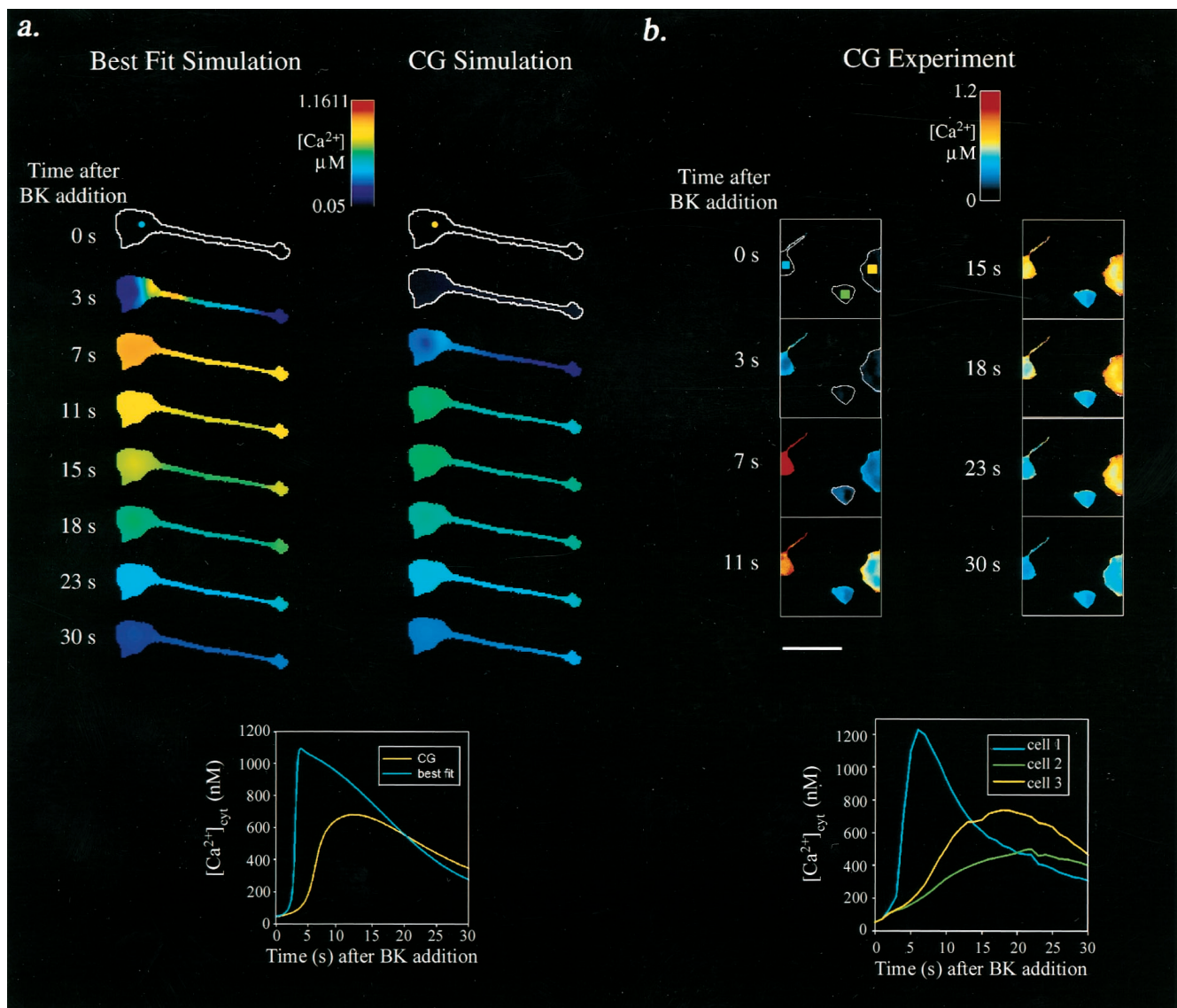
FIGURE 5 (a) Best-fit calcium simulation results for the cell shown in Fig. 1 (first column) and best fit simulation with 100 \mu\text{M} additional CG-10 kD dextran (second column). [Ca^{2+}]_{\text{cyt}} versus time is plotted below for points in the soma (cyan and yellow circles in the 0 s images). (b) Experimental results of a BK-induced calcium wave for three cells: cells 2 and 3 have been microinjected with 100 \mu\text{M} CG-10 kD dextran. Cells were loaded with fura-2/AM; 340/380-nm ratio pairs were collected every second, and converted to [Ca^{2+}] . [Ca^{2+}]_{\text{cyt}} versus time is plotted below for regions of interest in the somas (cyan, green, and yellow rectangles in the 0 s images). Scale bar = 100 \mu\text{m} .
