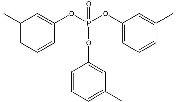
Tri-m-cresyl phosphate
