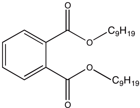
Diisononyl phthalate
