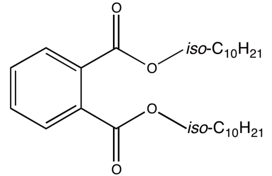
Diisodecyl phthalate
