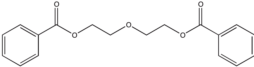
Diethylene glycol dibenzoate
