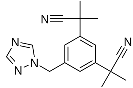
Anastrozole
