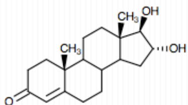
16- \alpha -hydroxytestosterone
