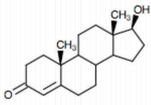
Testosterone
