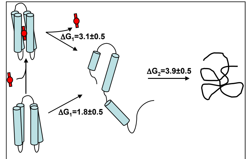
Model for the unfolding pathway of rop mutants with and without heme consistent with circular dichroism and fluorescence data.
