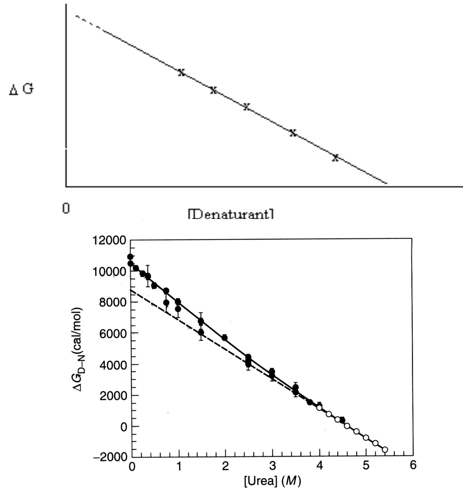
Figure 17.3 Urea denaturation of barnase at 25°C. The open circles were measured directly at 25°C from the ratios [D]/[N] , which were determined spectroscopically. The solid circles are values extrapolated to 25°C from thermal unfolding experiments at lower concentrations of urea and higher temperatures.
