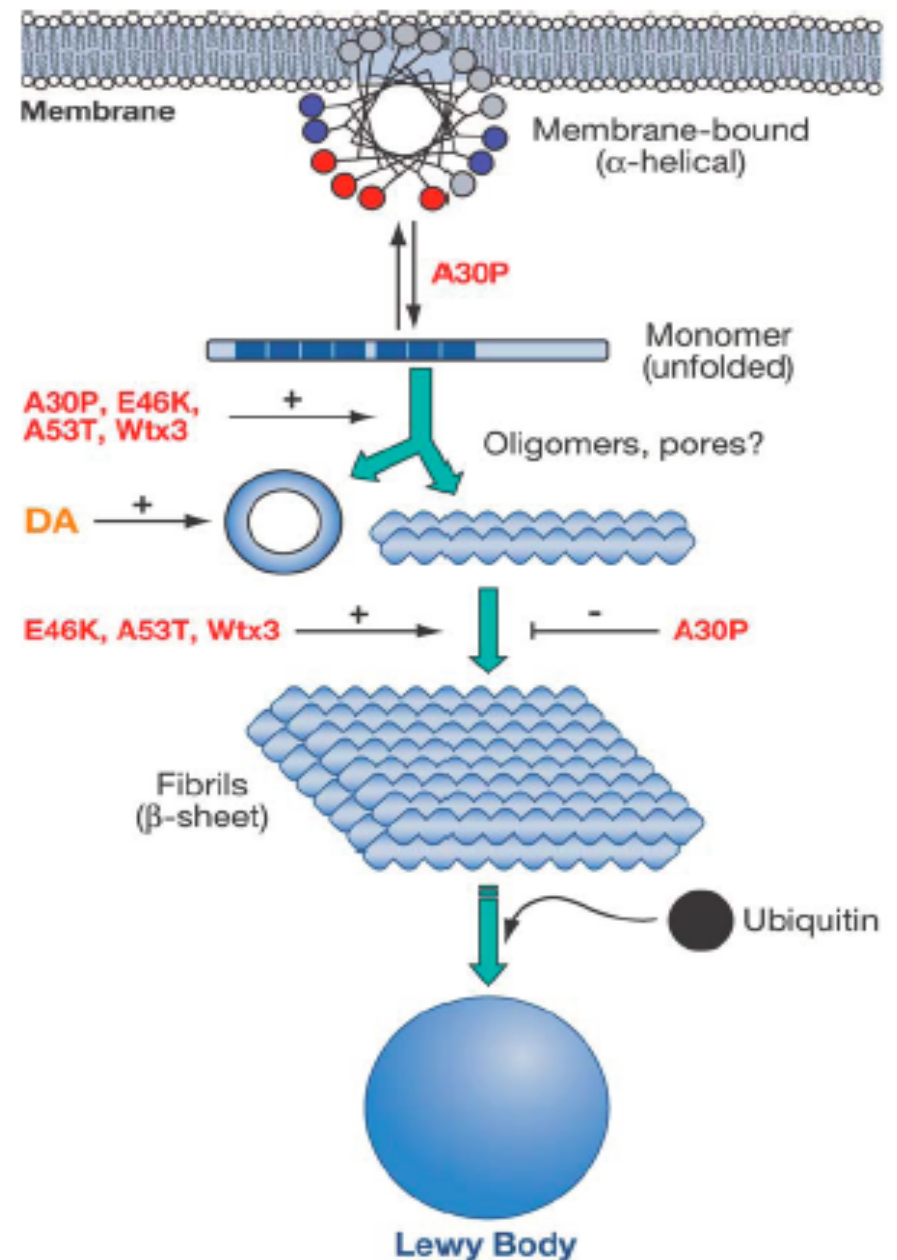
Figure 2 The pathogenic cascade of \alpha -synuclein aggregation. \alpha -Synuclein exists in solution as an unstructured monomer, shown as a linear structure, similar to Figure 1. Inside the cell, the monomer is in equilibrium with membrane-associated forms with higher helical content, shown schematically as an amphipathic helix. In the helix, blue and red circles indicate charged residues, gray circles are nonpolar and hydrophobic amino acids. The A30P mutation disfavors membrane binding. The green arrows indicate the pathogenic formation of aggregated species. All mutations reported to date increase the rate of formation of oligomers or protofibrils, which may also produce pores. Oligomers and other intermediates are kinetically stabilized by dopamine (DA). However, these are transient species that further aggregate to form mature fibrils, which are stabilized by \beta -sheet-like interactions and are highly insoluble. The formation of Lewy bodies is presumed to be a consequence of fibrillization. Events such as the attachment of ubiquitin ( black dot in the figure) are thought to be secondary to the initial aggregation and deposition processes.
