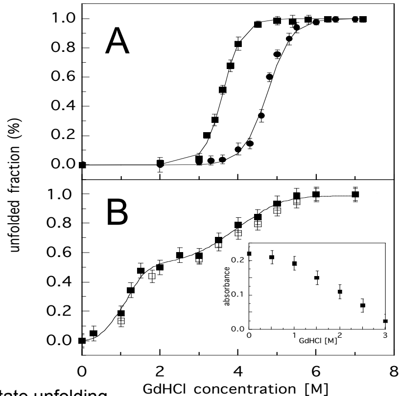
A: two state unfolding
