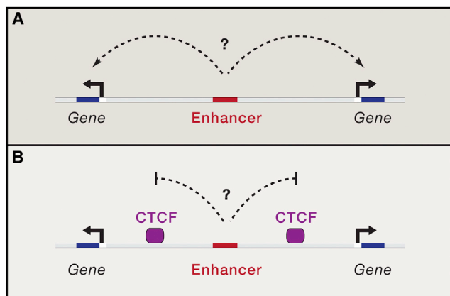
Figure 1. The Enhancer-Gene-Specificity Conundrum
