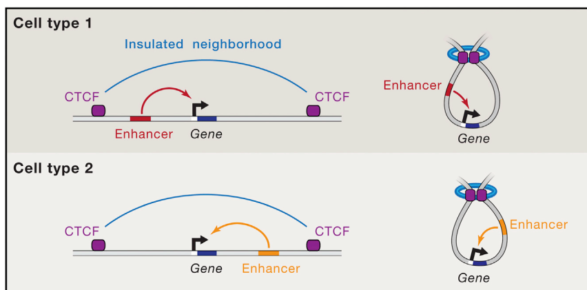
Figure 3. Insulated Neighborhoods in Development
