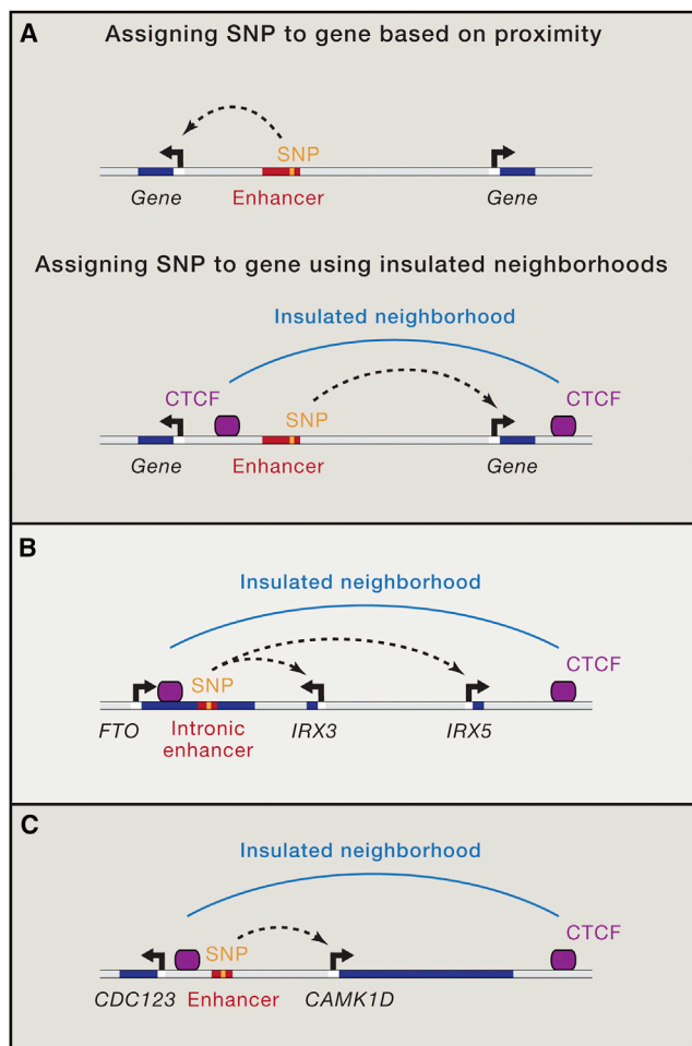
Figure 7. Insulated Neighborhoods as a Method to Identify Target Genes of Disease-Associated Enhancer Variation
