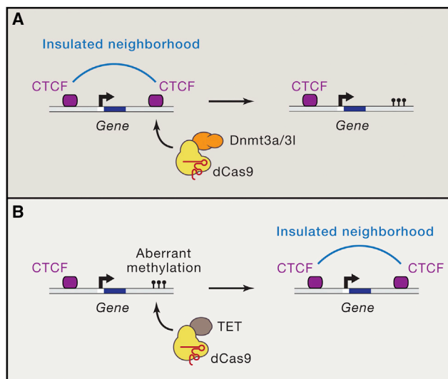
Figure 8. Neighborhood Perturbation and Repair through Site-Specific DNA Methylation
