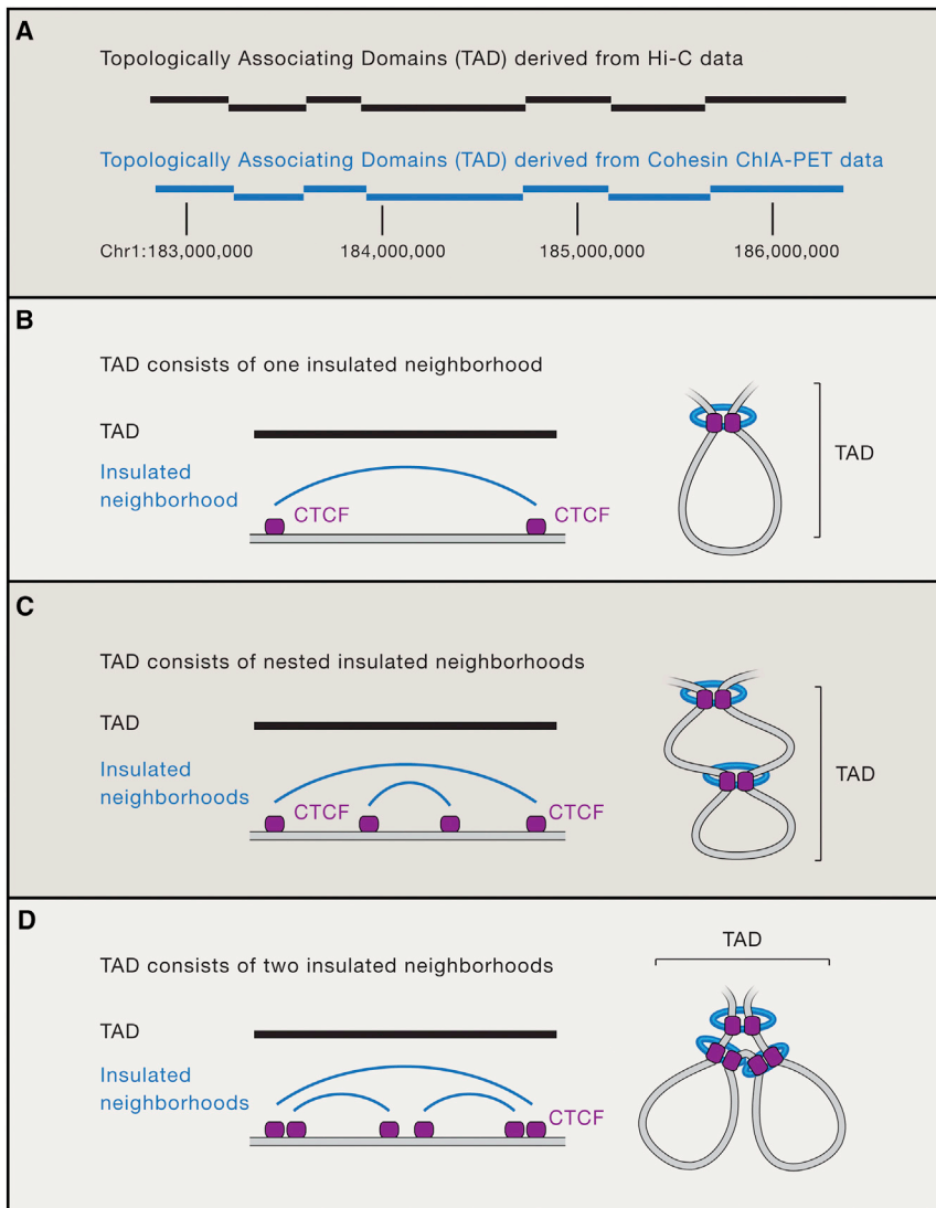
Figure 4. Insulated Neighborhoods Are the Mechanistic Basis of TADs
