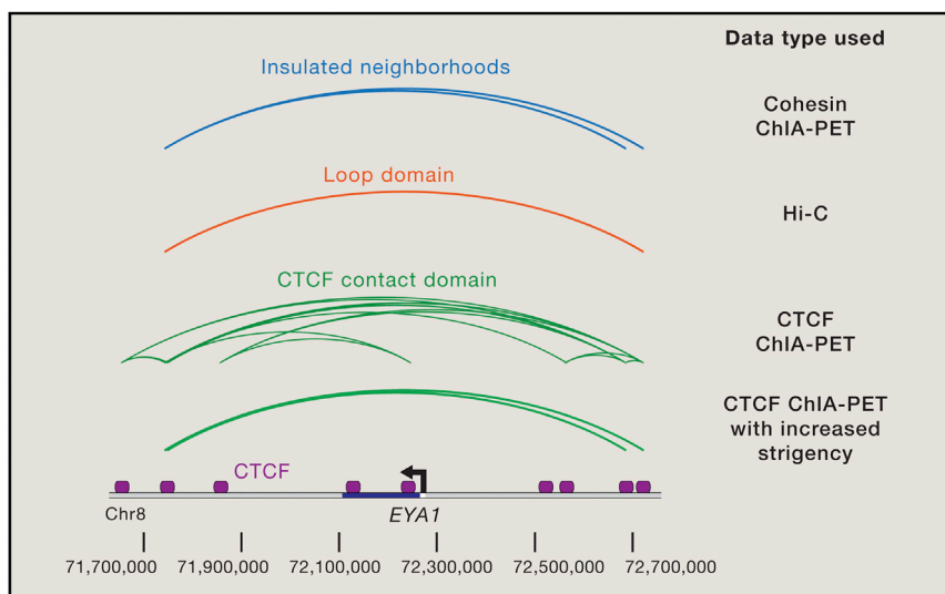
Figure 5. Relationships between Insulated Neighborhoods and Other DNA Loop Models
