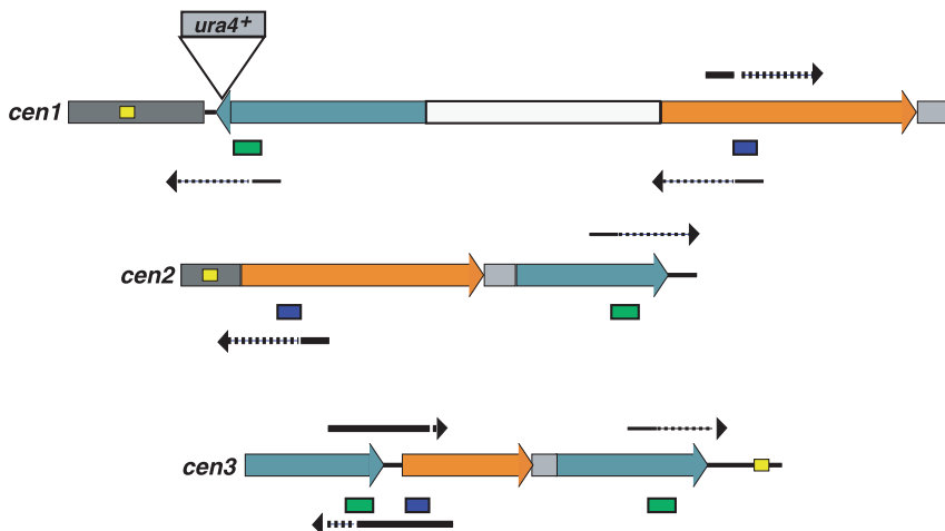
Fig. 5. One repeat unit from each of the three centromeres is shown (see Fig. 1). Transcripts from ago1 - mutant cells were identified by sequencing RT-PCR and RACE-PCR products, and those unique to each centromere are shown as thick arrows. Transcripts whose origin was ambiguous due to sequence identity between the centromeres are shown as thin arrows. Transcript length, determined by Northern blots (Fig. 1), allowed us to estimate the approximate position of the transcribed region (indicated by dashed lines). The PCR product that detected run-on dh repeat transcription toward the centromere in wild-type cells (Fig. 3) is indicated as a blue bar. The PCR product amplified in ChIP experiments with K9 and K4 antibodies (Fig. 3A) as well as with rdp-HA antibodies (Fig. 4) is indicated as a green bar underneath each dg repeat. A similar PCR product was used as the probe for the Northern blot shown in Fig. 1.
