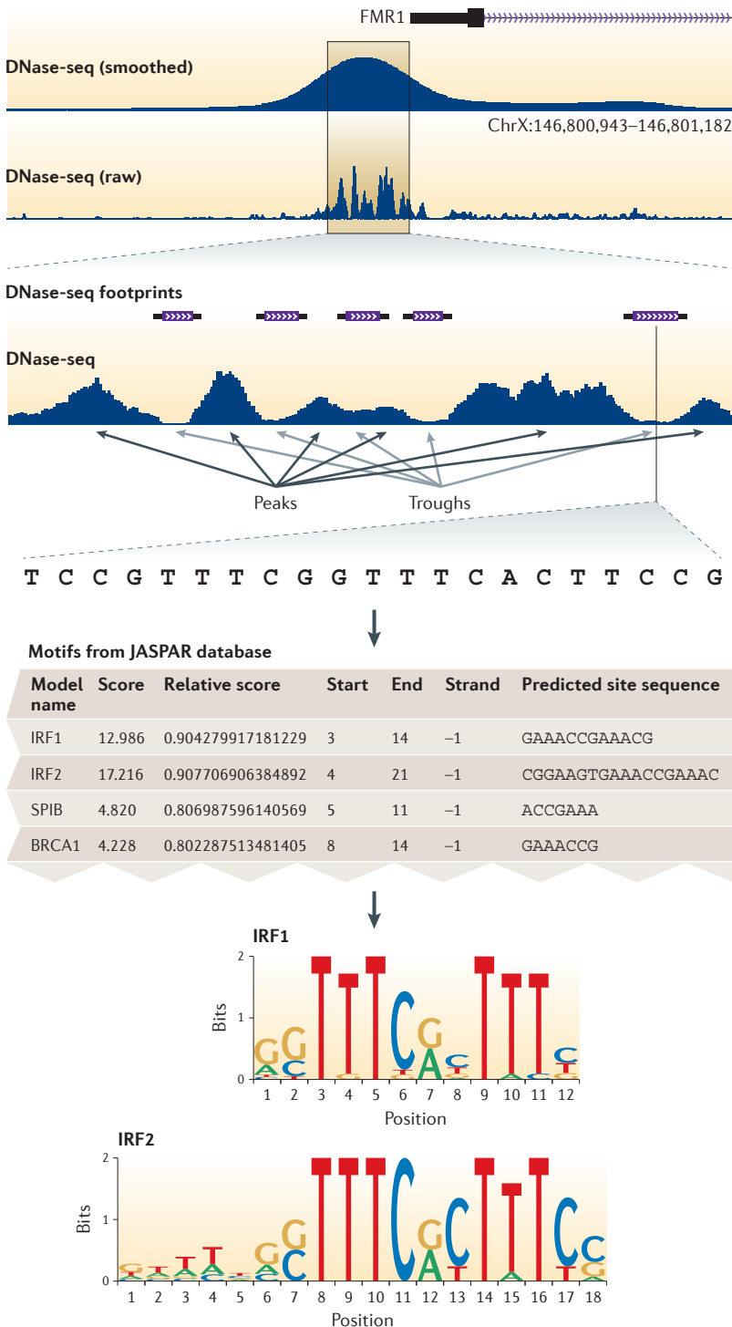
Figure 3 | DNaseI footprints correspond to bound proteins. The distribution of DNaseI digestion sites with DNaseI hypersensitive regions is not uniform; peaks and troughs occur in the signal, where troughs are due to the protection of DNA sequences by bound proteins. Transcription factor binding motif databases such as JASPAR 81 can be searched using the sequence from each footprint to predict what factor is bound. Shown here are data from the proximal promoter region of the human fragile-X mental retardation 1 ( FMR1 ) gene, with motif-matching results for one footprint indicating that potentially bound factors are interferon regulatory factor 1 (IRF1) or IRF2. DNaseI footprints had been identified previously at this locus 110 in lymphoblastoid cells. More recent data from DNase-seq was used to recapitulate these results in a single experiment 12 . The upper panel is modified, with permission, from REF 12 © (2010) Cold Spring Harbor Laboratory Press.
