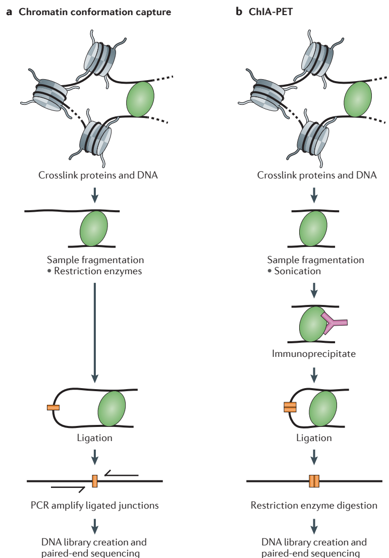
Figure 4 | Detecting chromatin interactions. In three-dimensional space, distal genomic regions on the same or different chromosomes interact, and this can be mediated by one or more DNA-binding proteins. a | Chromatin conformation capture experiments use a ligation step to join distant fragments that are interacting in three-dimensional chromatin space, thus providing information on possible targets for DNA-bound proteins. b | Chromatin interaction analysis with paired-end tag sequencing (ChIA-PET) similarly detects chromatin interactions using a ligation step to pair non-adjacent interacting regions. However, ChIA-PET uses a chromatin immunoprecipitation (ChIP) step to more specifically identify interactions with a particular bound protein, such as RNA polymerase II. It should be noted that the DNA that is actually sequenced as part of the paired-end sequencing does not necessarily correspond to the precise region of interaction but is dictated by the presence of restriction enzyme targets.
