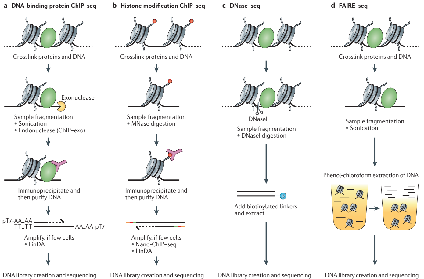
Figure 1 | Comparison of experimental protocols. Experiments to detect different aspects of DNA-binding proteins share many of the same steps; simplified schematics of the main steps are shown. a | Chromatin immunoprecipitation followed by sequencing (ChIP-seq) for DNA-binding proteins such as transcription factors. Recent variations on the standard protocol include using endonuclease digestion instead of sonication (ChIP-exo) to increase the resolution of binding-site detection and to eliminate contaminating DNA, and DNA amplification after ChIP for samples with limited cells. b | ChIP-seq for histone modifications uses micrococcal nuclease (MNase) digestion to fragment DNA and can also now be run on low-quantity samples when combined with the additional post-ChIP amplification. c | DNase-seq relies on digestion by the DNaseI nuclease to identify regions of nucleosome-depleted open chromatin where there are binding sites for all types of factors, but it cannot identify what specific factors are bound. d | Formaldehyde-assisted identification of regulatory elements (FAIRE-seq) similarly identifies nucleosome-depleted regions by extracting fragmented DNA that is not crosslinked to nucleosomes. LinDA, single-tube linear DNA amplification; T7, T7 phage RNA polymerase.
