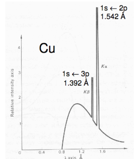
FIGURE A4.3. Characteristic K spectrum superposed on the "white" radiation continuum.
